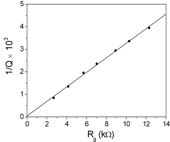
Fig. 2: Inverse of the resonator quality factor 1/Q as function of the ground resistor R_g . The straight line is the best linear fit to the experimental data.
