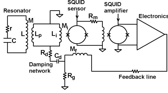
Fig. 1: Circuit diagram of the closed loop two-stage dc SQUID coupled to the high Q electrical resonator. The capacitive damping network is also shown.
