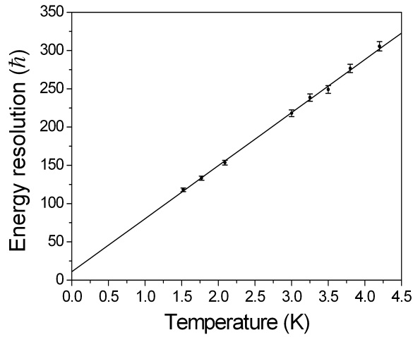
Fig. 3: Energy resolution in the white noise region of the SQUID coupled to the high Q resonator. The straight line is the best weighted linear fit to the experimental data.
