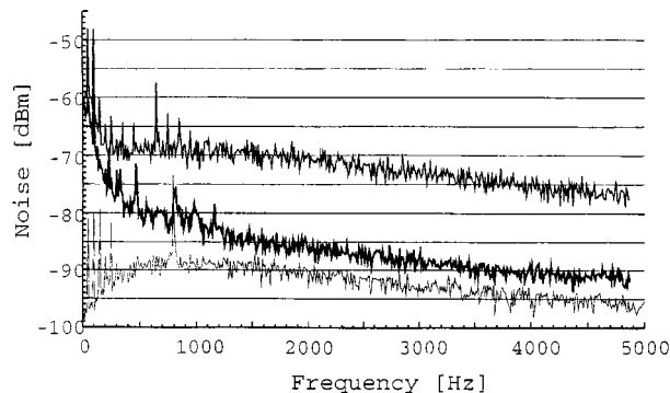
Fig. 7. Same spectra as in Fig. 6, measured after the optical fiber for 15-mW laser power.
