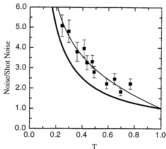
Fig. 5. Ratio of intensity noise spectral density to shot noise, as a function of the transmissivity of BS1. The experimental data are fitted with Eq. (9). Thick curve, theoretical limit for infinite gain.
