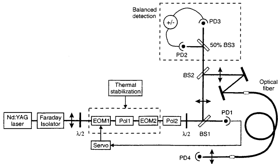
Fig. 1. Experimental setup: \lambda/2 , half-wave plate; Pol, polarizer.
