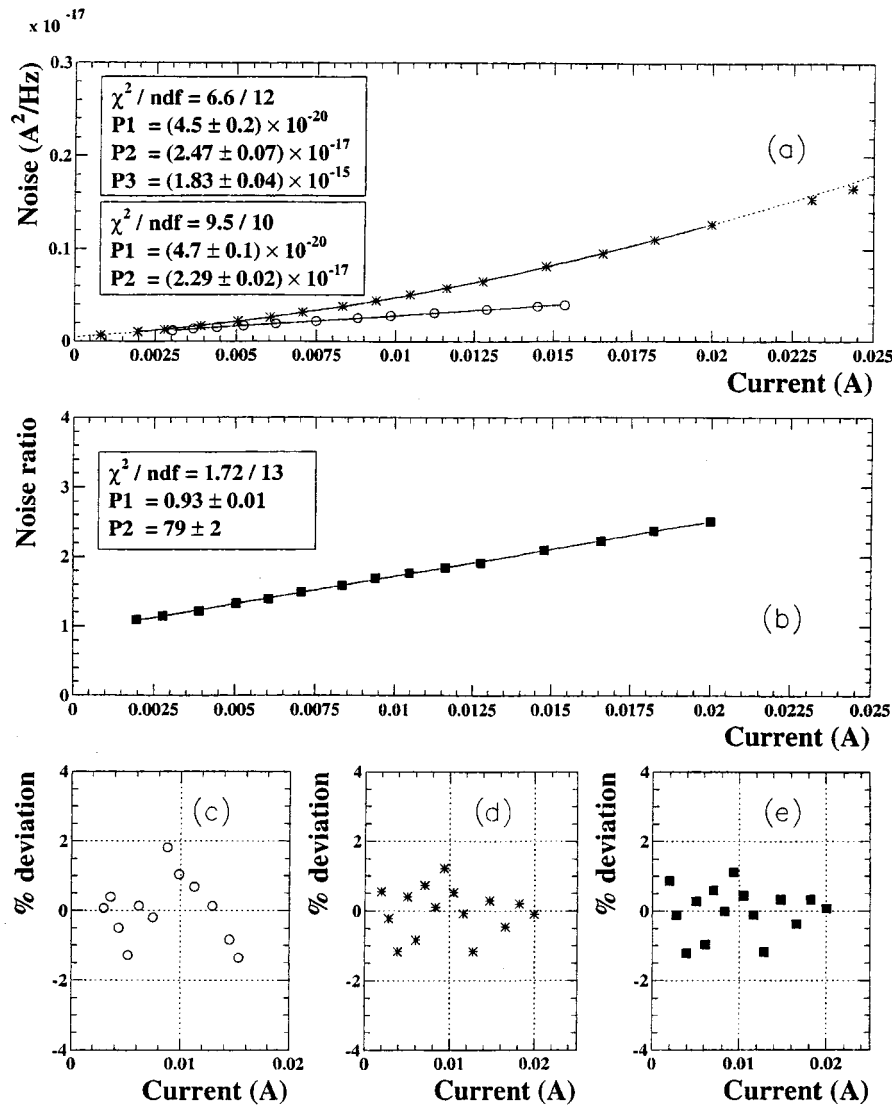
Fig. 3. (a) Power spectral density at 10 MHz of the intensity noise as a function of the photocurrent generated by a halogen lamp (lower curve, fitted with a straight line) and by the laser (upper curve, fitted with a second-order polynomial). P1, P2, and P3 are the coefficients of the zero-, first-, and second-order terms in the fitting function, respectively. (b) Laser power density normalized to shot noise as a function of the photocurrent. Percentage deviations from the fitting curves are shown on the bottom: (c) halogen lamp, (d) laser, (e) noise ratio.
