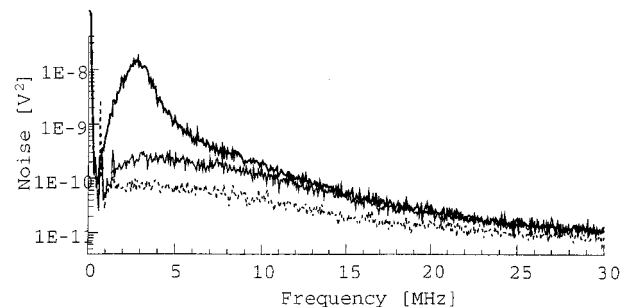
Fig. 2. Upper curve, intensity noise power for 9 mW impinging on the detector; middle curve, shot-noise calibration obtained with a halogen lamp; lower curve, detector electronic noise.
