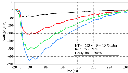
Figure 3: Amplificated signals (50Ω adapt.).
