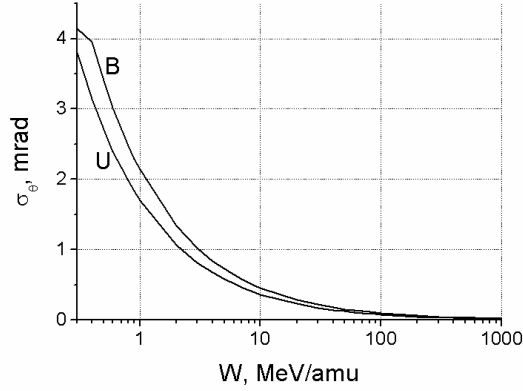
Figure 7: Dependence of the scattering angles for B and U in the carbon foils having the equilibrium thickness.
