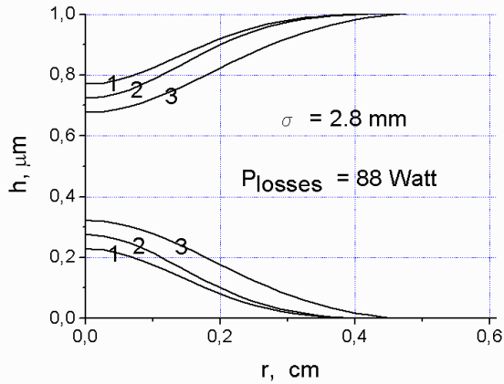
Figure 11: Curves 1,2, and 3 correspond accordingly to the moment 100 c, 200 c and 2000 c after beginning of irradiation.
