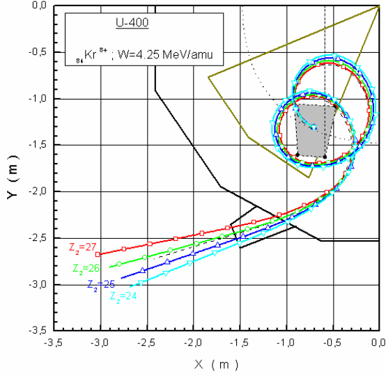
Figure 1: Two-turn extraction from U400 cyclotron.
