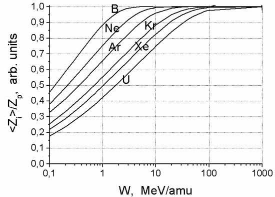
Figure 5: Dependence of the ion stripping degree on the ion energy.
