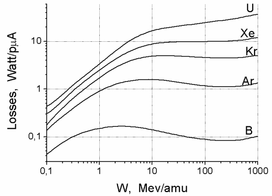
Figure 9: Power losses of the ion beam.
