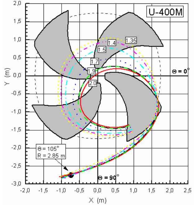
Figure 2: Reference particle trajectories of the ions extracted from U400M cyclotron by method 2.
