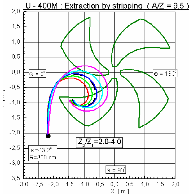
Figure 3: Trajectories of the low energy ion beams extracted from U400M cyclotron by method 1.
