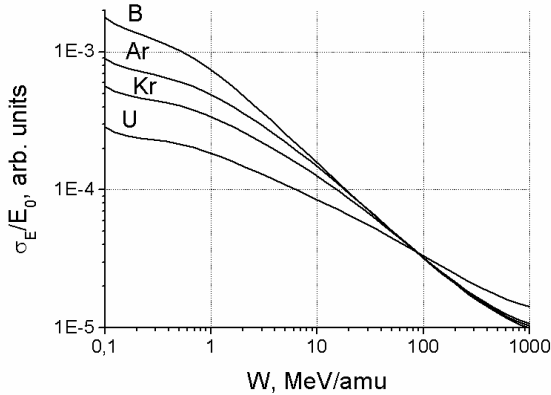
Figure 8: Dependence of the additional energy spread in the extracted beam.
