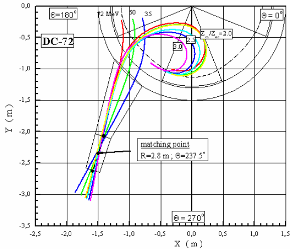
Figure 4: Reference particle trajectories of the ions extracted from DC72 cyclotron.
