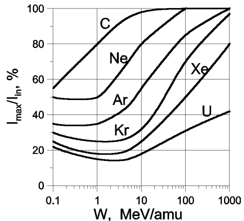
Figure 6: Maximum efficiency of a single charge extraction by stripping.
