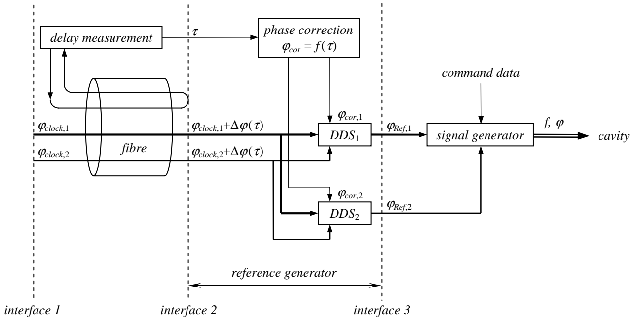
Figure 4: Generation of the reference signals.
