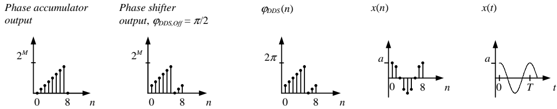
Figure 3: Direct digital synthesis principle.
