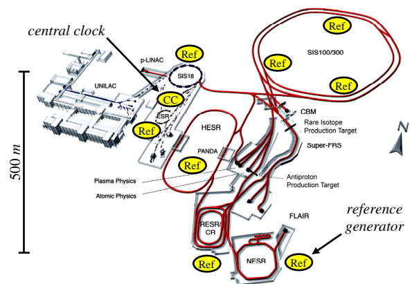
Figure 1: Facility for Antiproton and Ion Research.
