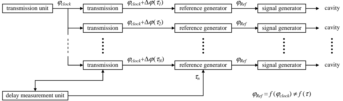
Figure 2: Basic principle of the cavity synchronisation.
